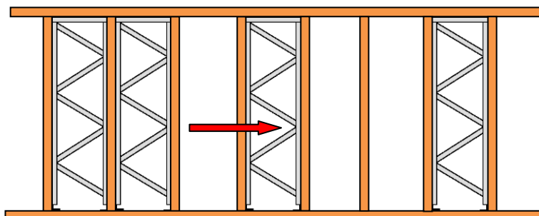
Figure 2: New Design layout with the 3 Gamma Frame re-positioned in the wall.
