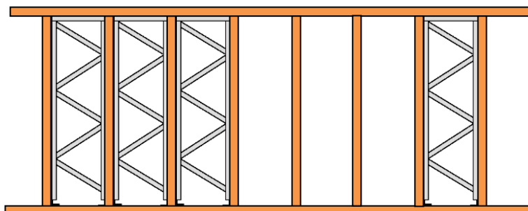
Figure 1: Original Design Layout
