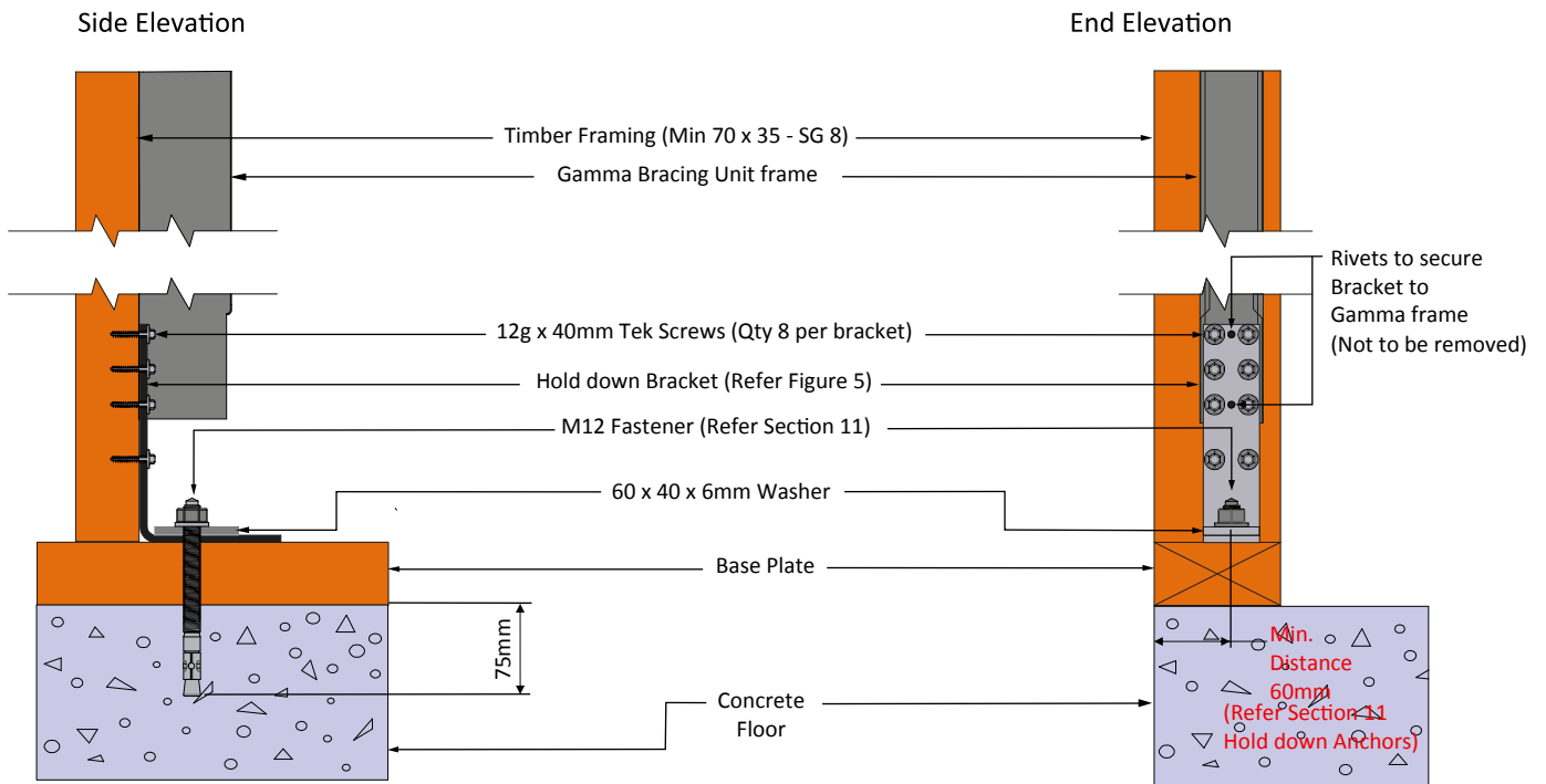
Figure 1 Hold Down Construction detail for Concrete Flooring
