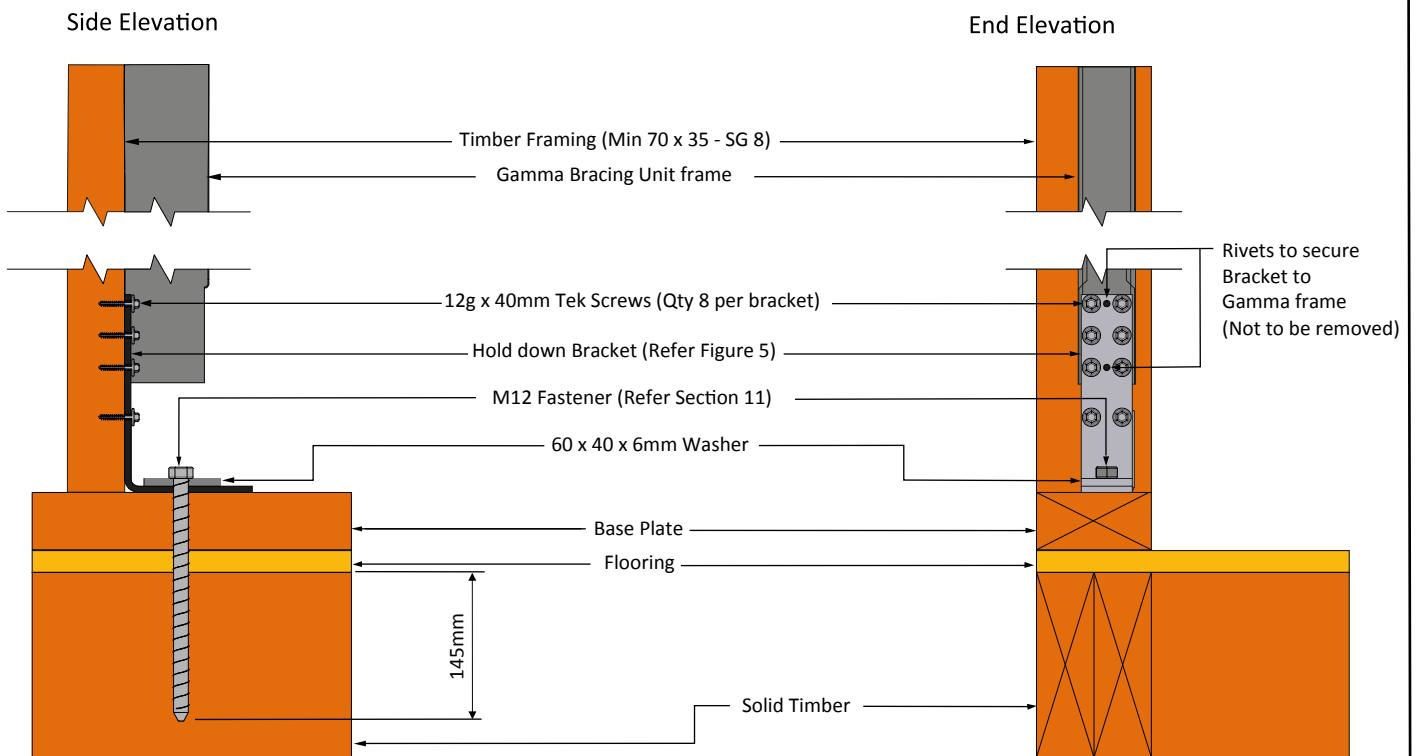
Figure 2 Hold Down Construction detail for Timber Flooring
