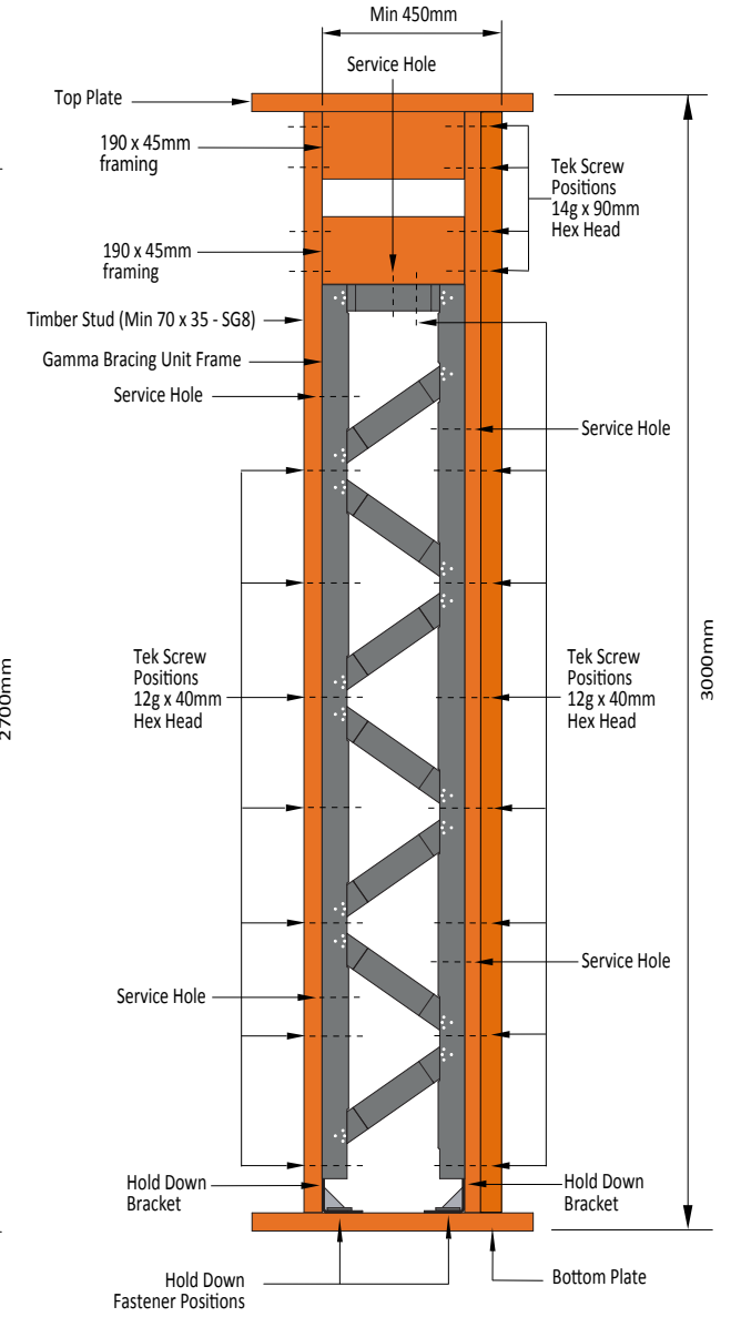
3.0m Wall Height
